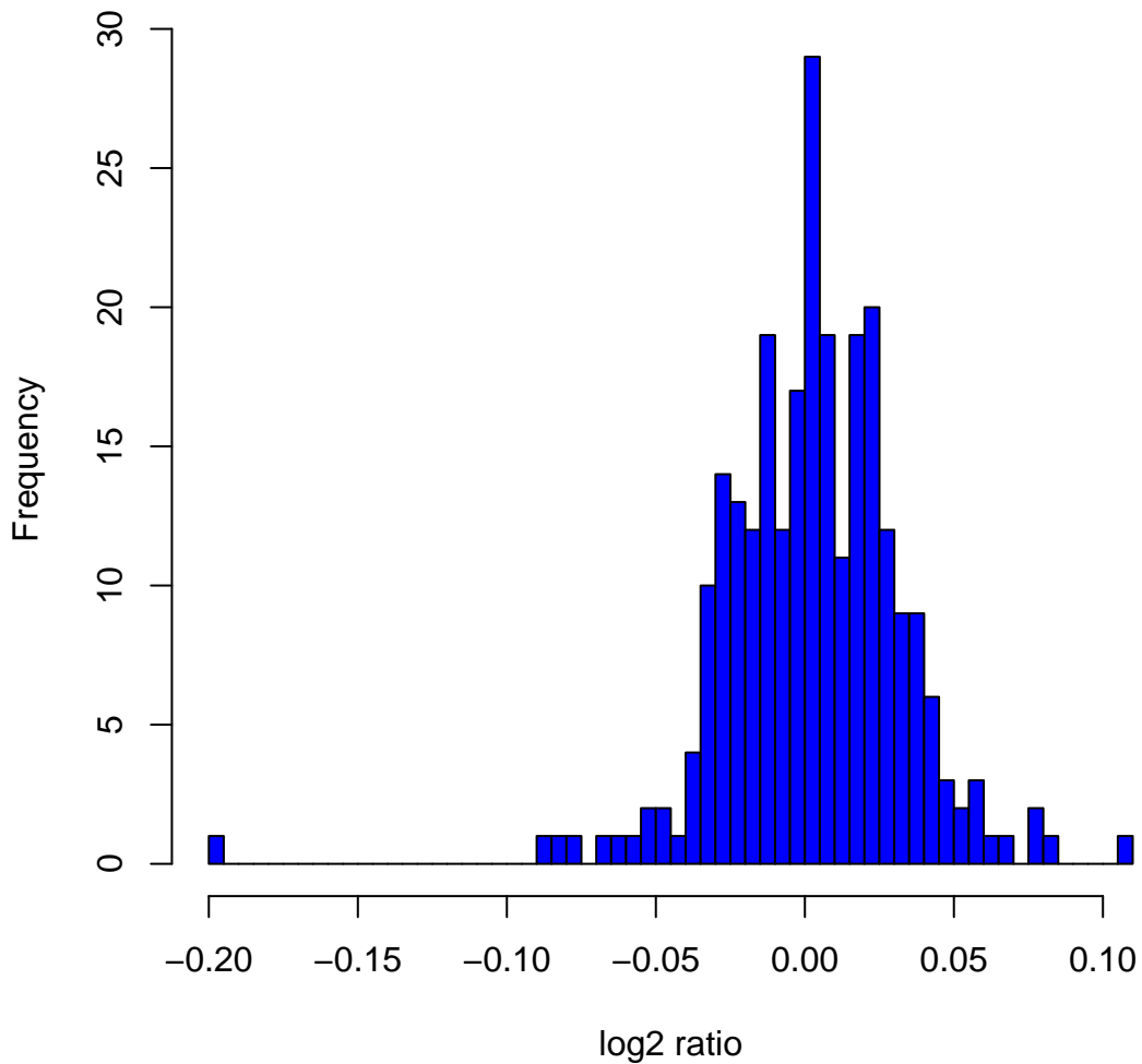
Histogram of log 2 ratios in 270 HapMap samples at clone Chr8tp-7D2
