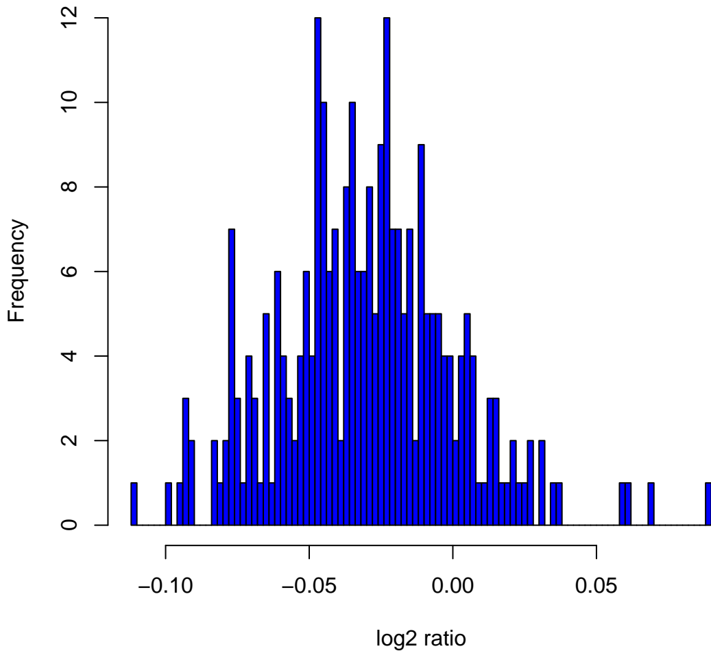
Histogram of log 2 ratios in 270 HapMap samples at clone Chr8tp-7E2
