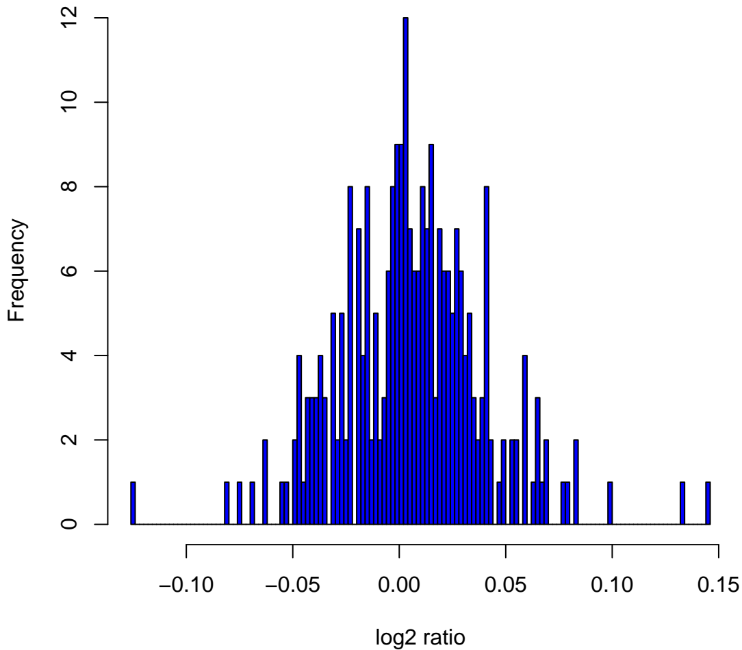
Histogram of log 2 ratios in 270 HapMap samples at clone Chr8tp-7E4
