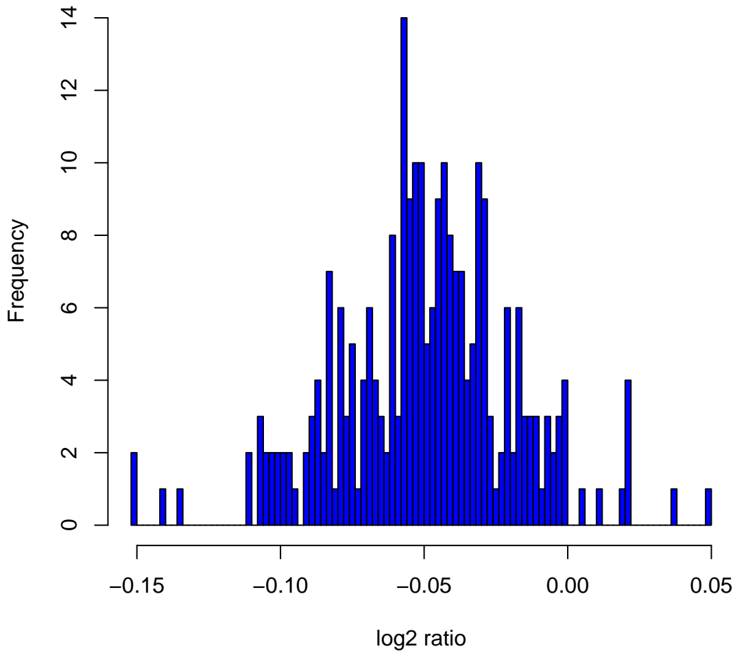
Histogram of log2ratios in 270 HapMap samples at clone Chr8tp-7F8
