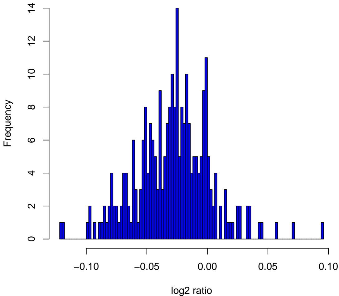
Histogram of log2ratios in 270 HapMap samples at clone Chr8tp-7F9
