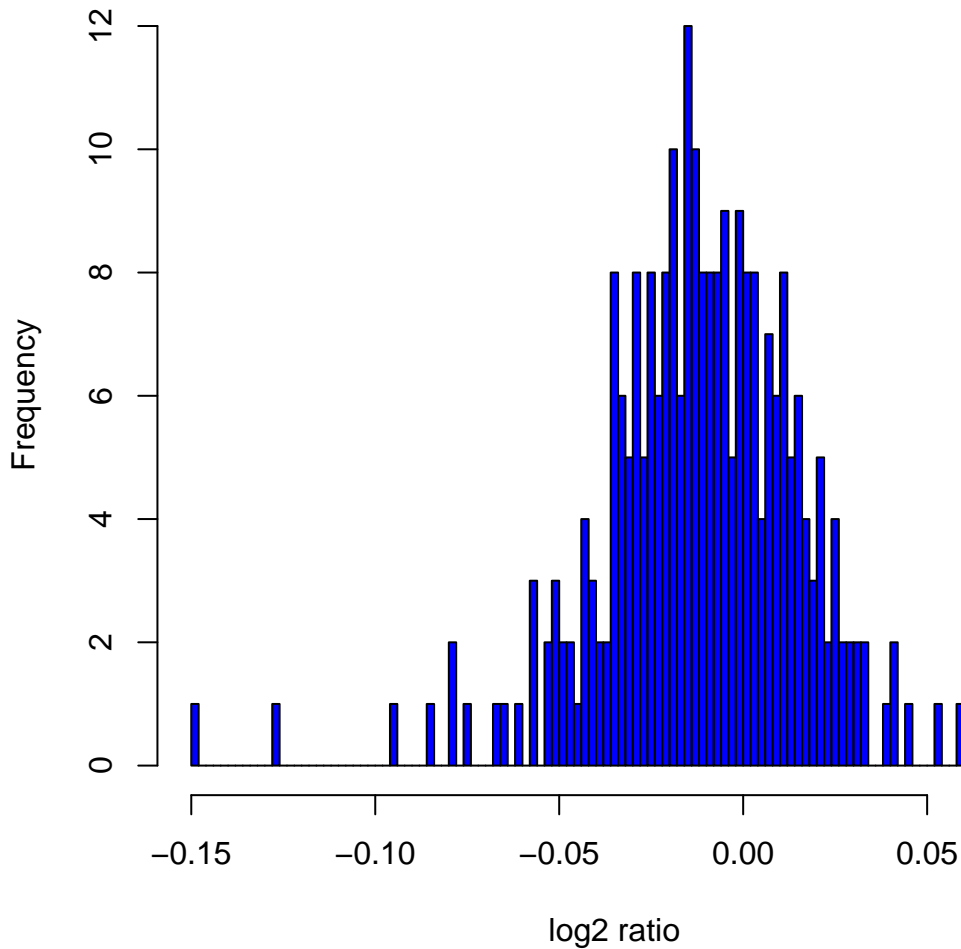
Histogram of log 2 ratios in 270 HapMap samples at clone Chr8tp-7H1
