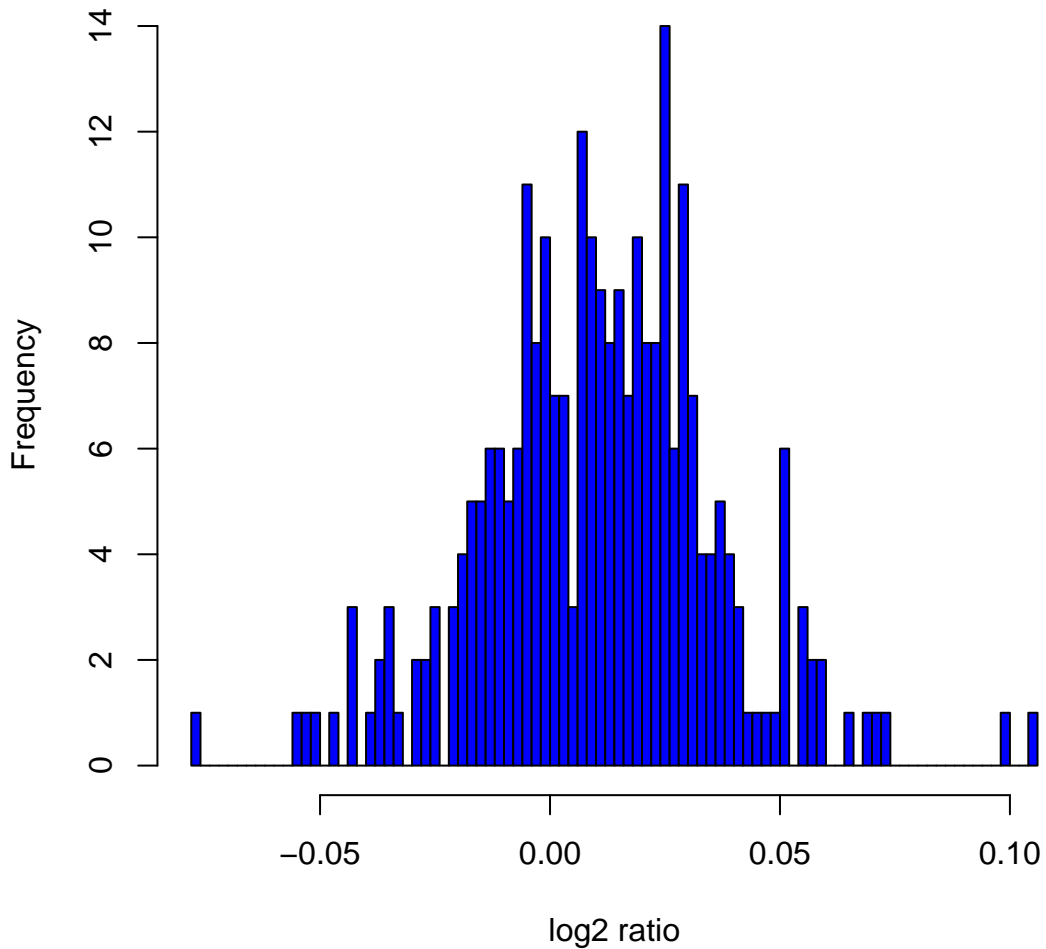
Histogram of log 2 ratios in 270 HapMap samples at clone Chr8tp-9A4
