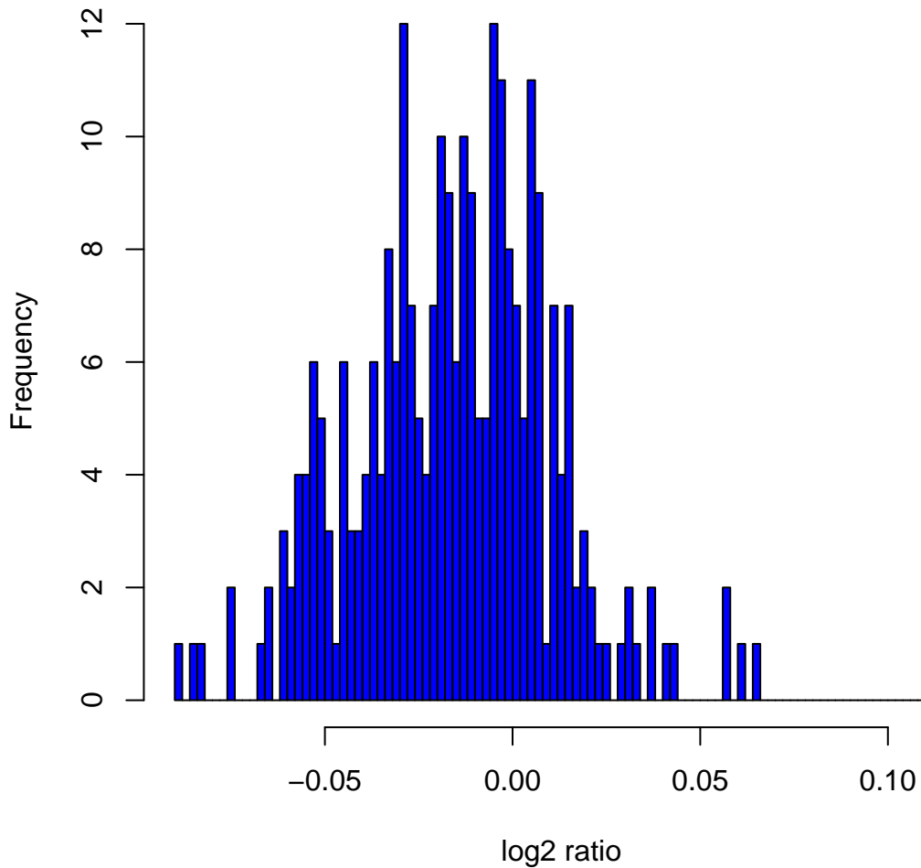
Histogram of log 2 ratios in 270 HapMap samples at clone Chr8tp-9C4
