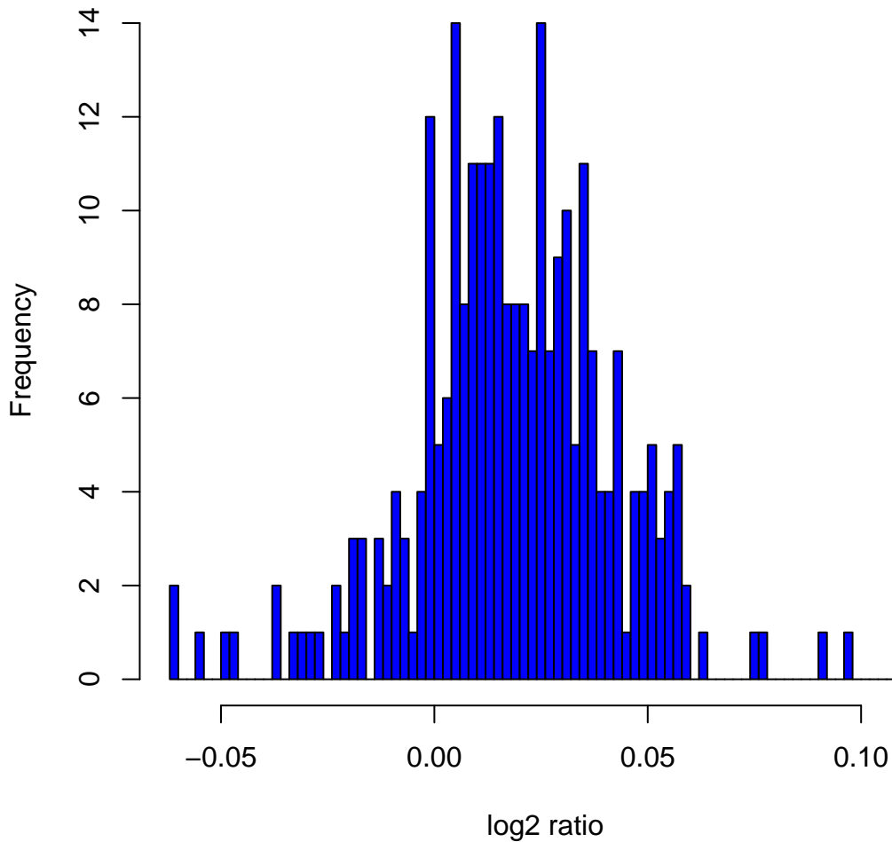
Histogram of log 2 ratios in 270 HapMap samples at clone Chr8tp-9C9
