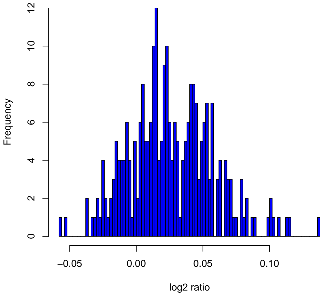
Histogram of log 2 ratios in 270 HapMap samples at clone Chr8tp-9D1
