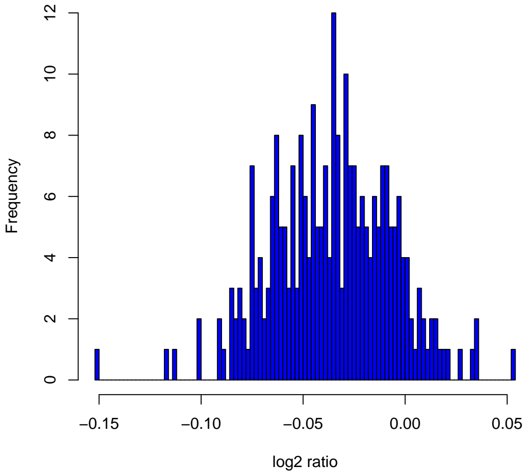
Histogram of \log_2 ratios in 270 HapMap samples at clone Chr8tp-9D7
