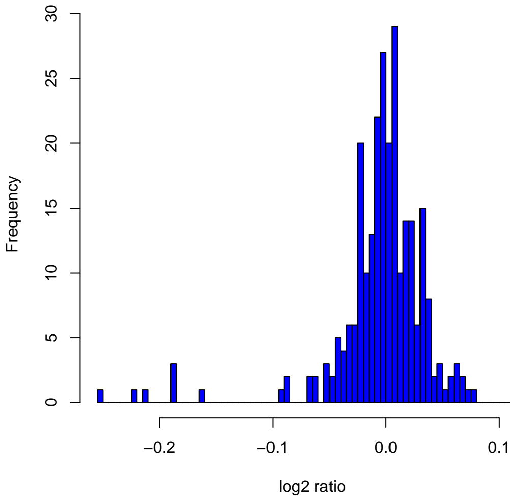
Histogram of log 2 ratios in 270 HapMap samples at clone Chr8tp-9E11
