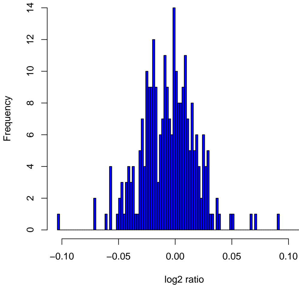
Histogram of \log_2 ratios in 270 HapMap samples at clone Chr8tp-9E5
