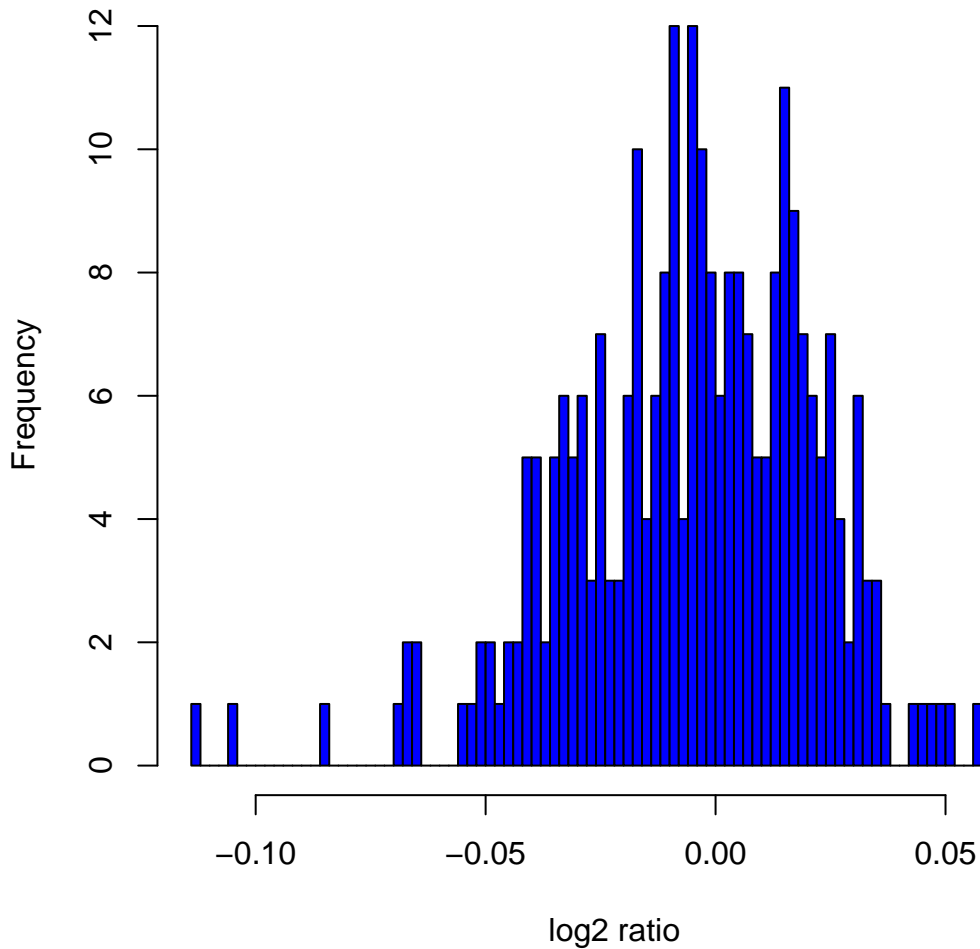
Histogram of log 2 ratios in 270 HapMap samples at clone Chr8tp-9E7
