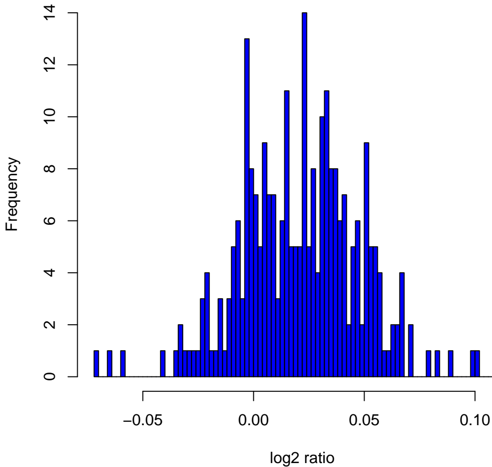
Histogram of \log_2 ratios in 270 HapMap samples at clone Chr8tp-9G6
