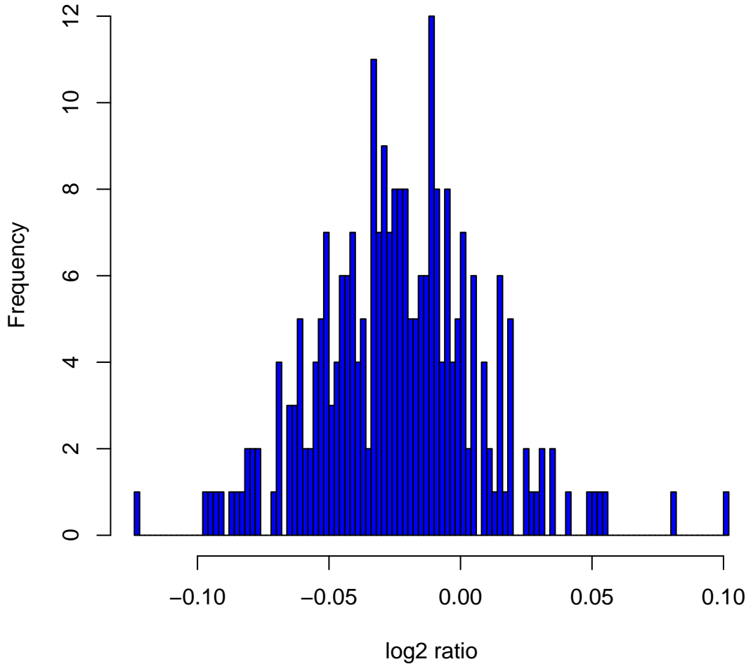
Histogram of log 2 ratios in 270 HapMap samples at clone Chr9tp-10C5
