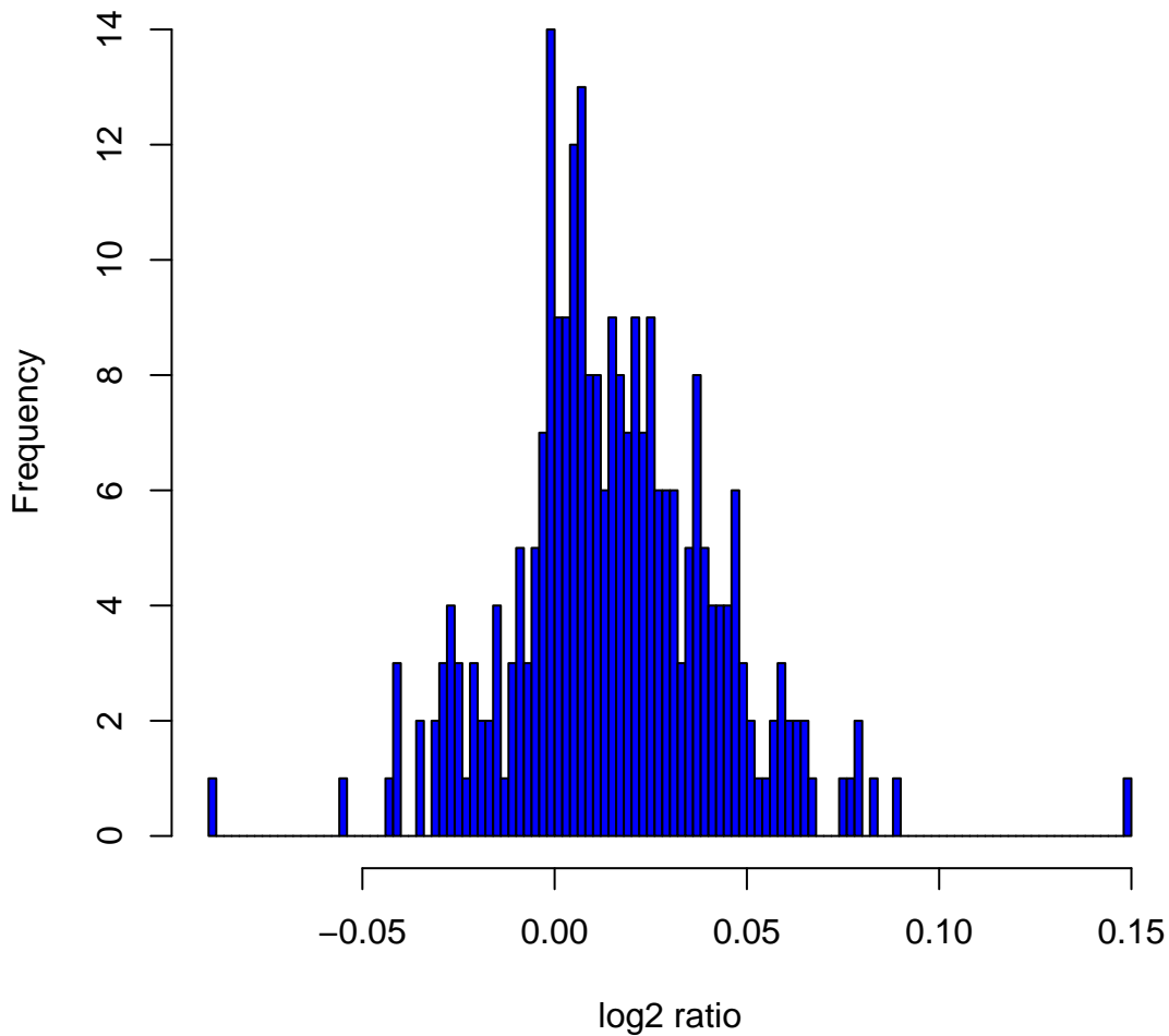
Histogram of log 2 ratios in 270 HapMap samples at clone Chr9tp-10D9
