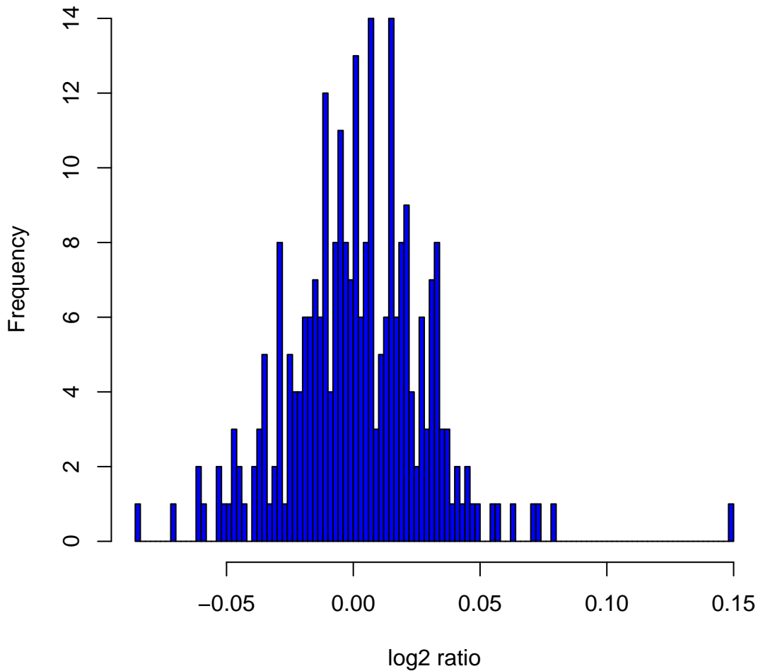
Histogram of log2ratios in 270 HapMap samples at clone Chr9tp-10E10
