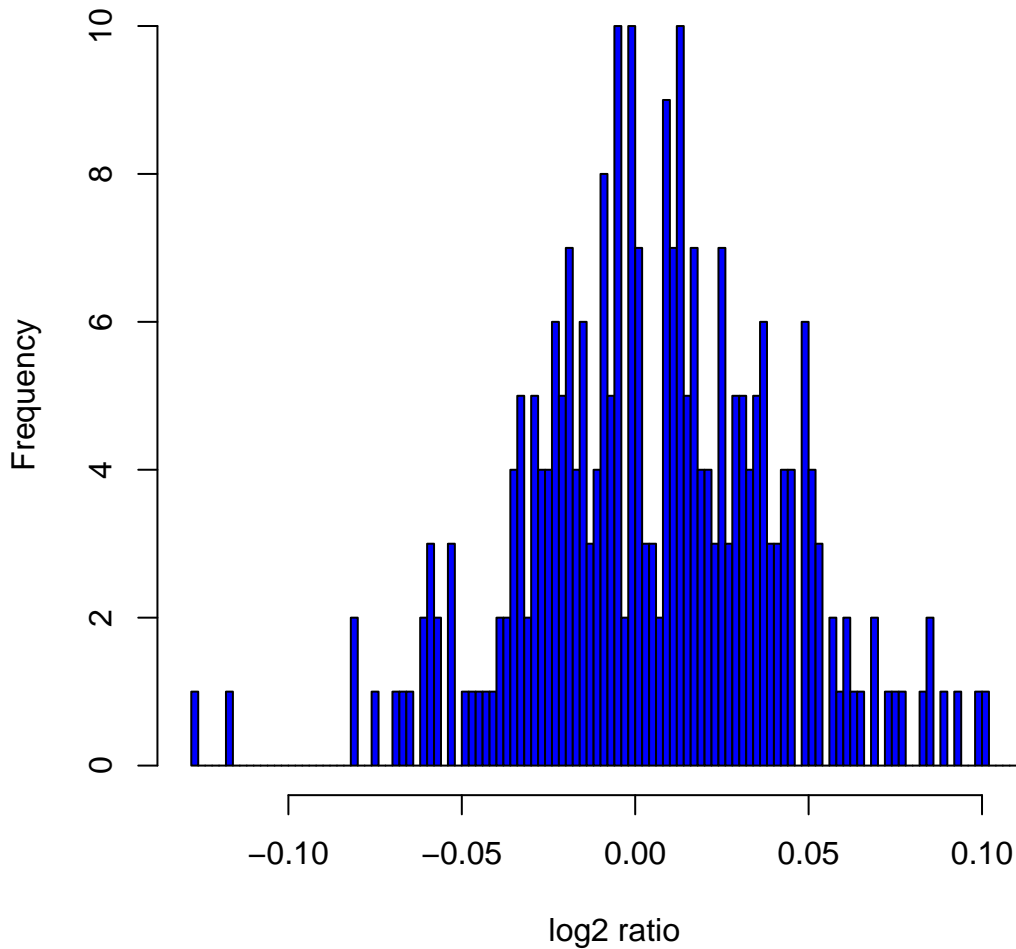
Histogram of log 2 ratios in 270 HapMap samples at clone Chr9tp-10E6
