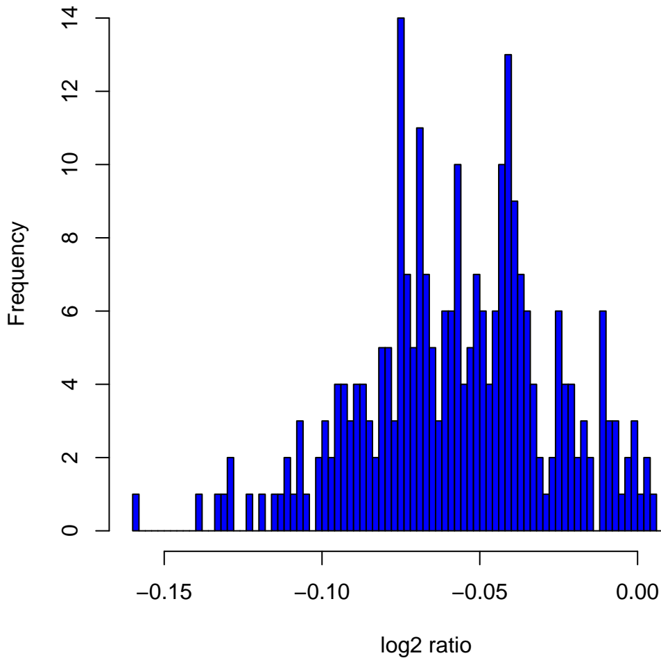
Histogram of log 2 ratios in 270 HapMap samples at clone Chr9tp-10G7
