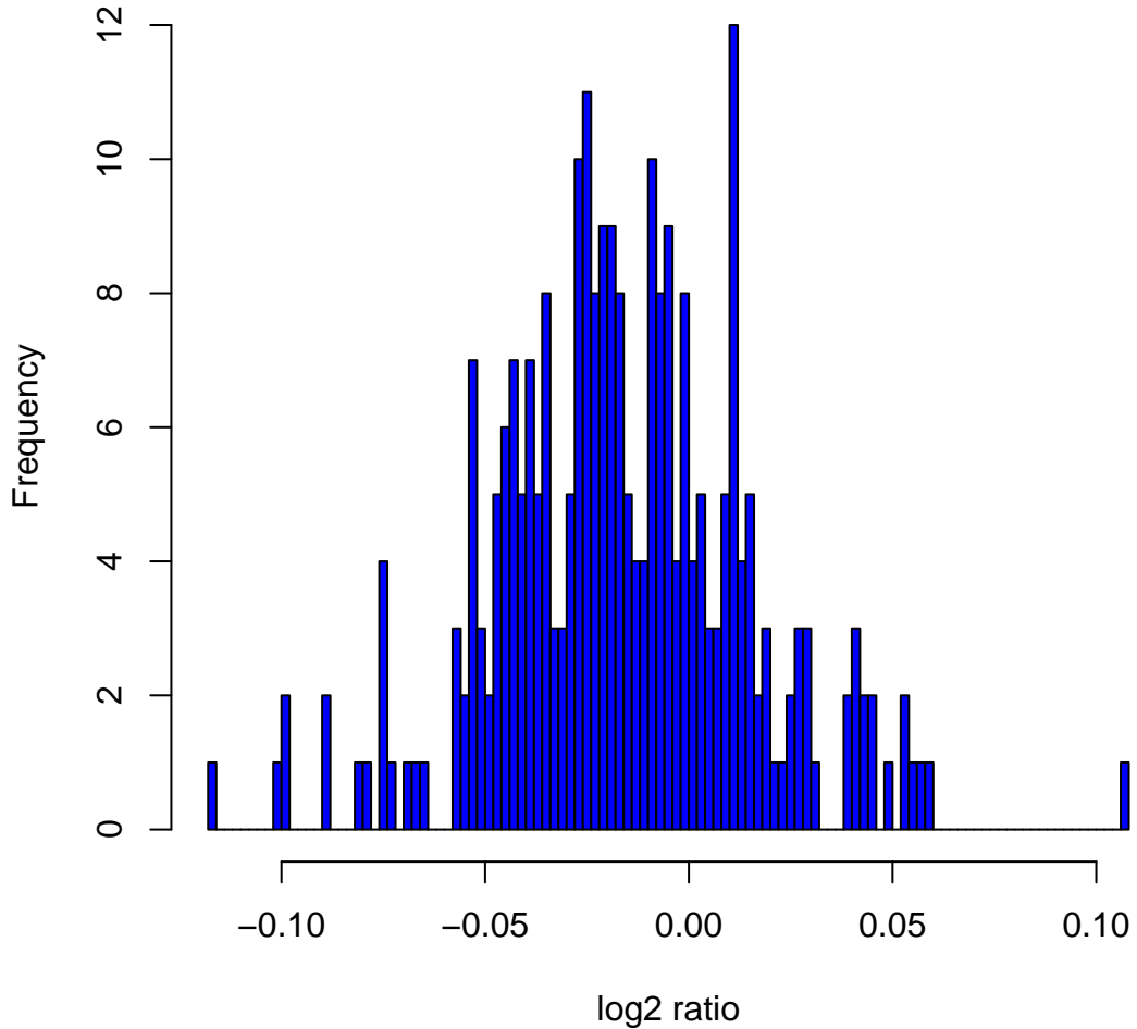
Histogram of log2ratios in 270 HapMap samples at clone Chr9tp-11A11
