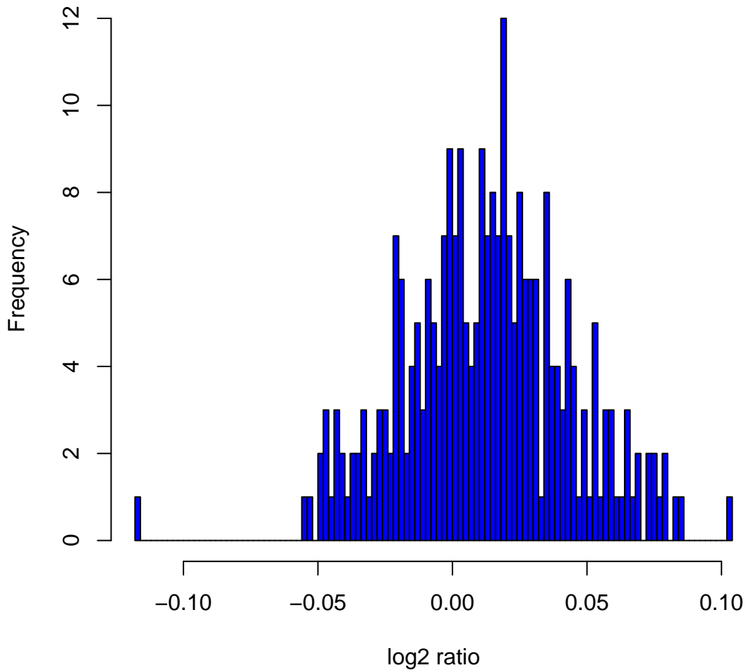
Histogram of log2ratios in 270 HapMap samples at clone Chr9tp-11B10
