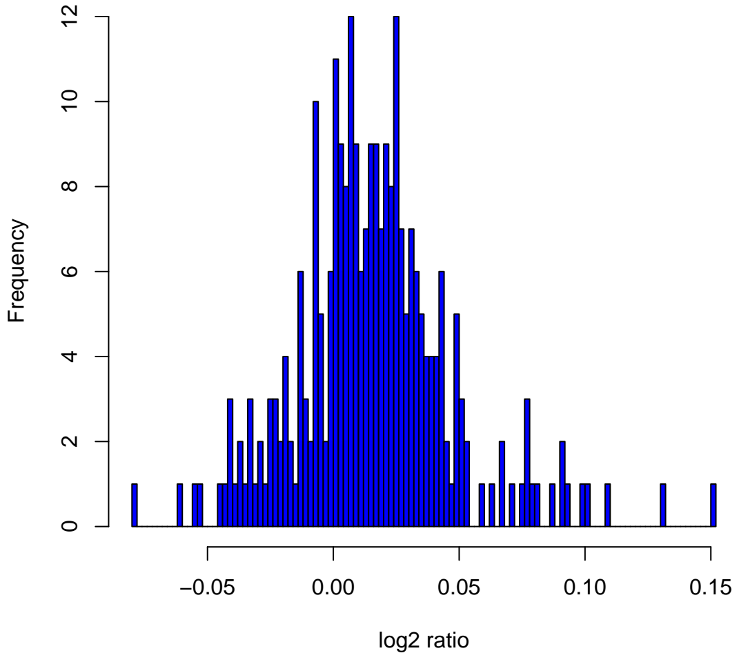
Histogram of \log_2 ratios in 270 HapMap samples at clone Chr9tp-11C7
