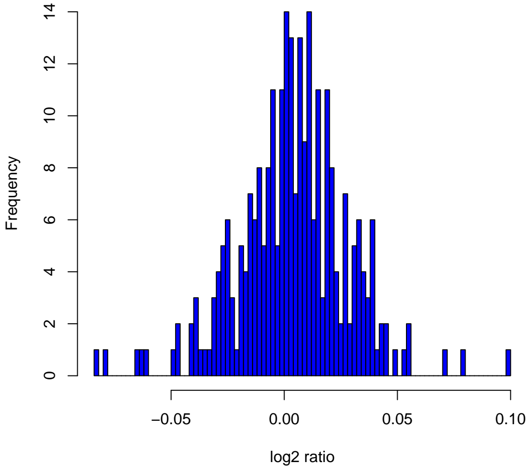
Histogram of log2ratios in 270 HapMap samples at clone Chr9tp-11E11
