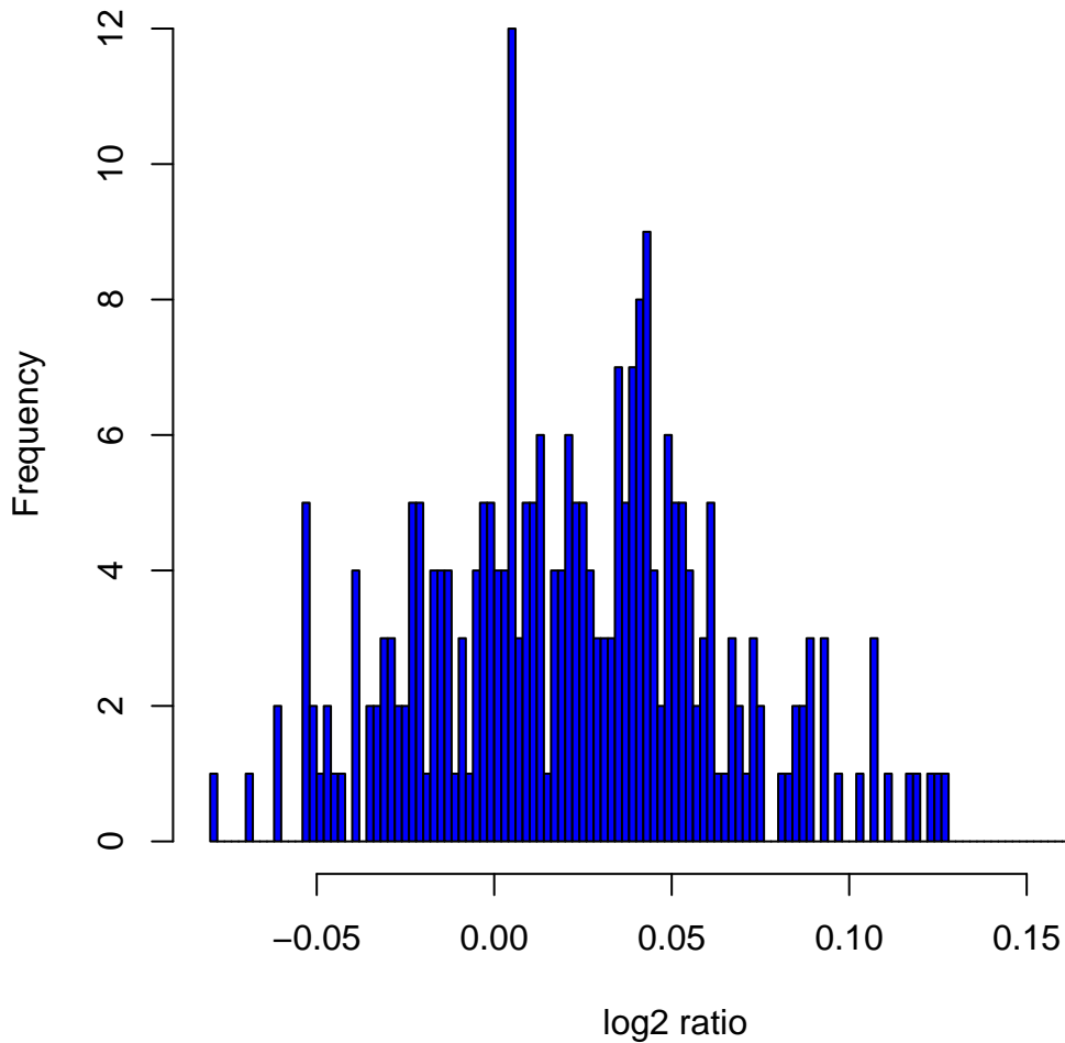
Histogram of log2ratios in 270 HapMap samples at clone Chr9tp-11H10
