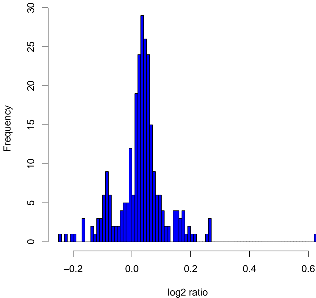
Histogram of log 2 ratios in 270 HapMap samples at clone Chr9tp-13D2
