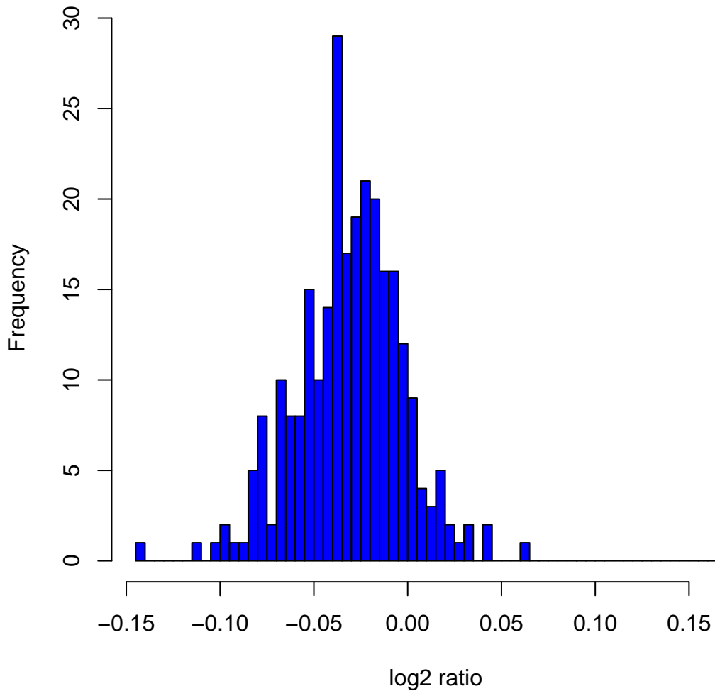
Histogram of log 2 ratios in 270 HapMap samples at clone Chr9tp-1C7
