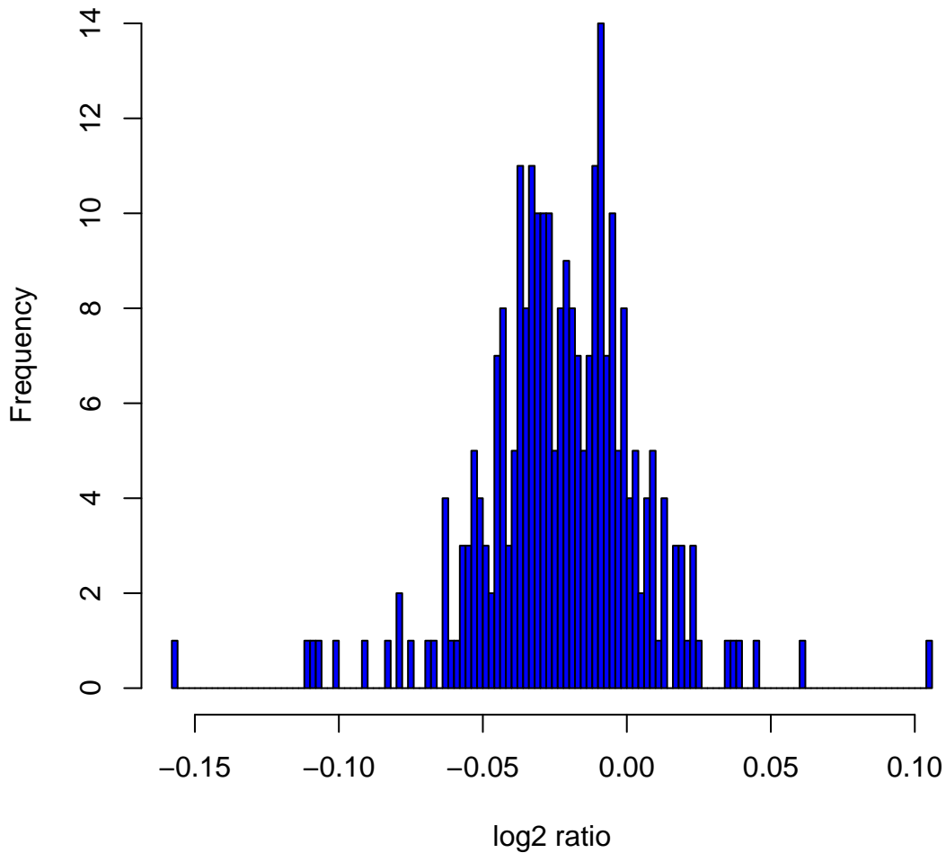
Histogram of log2ratios in 270 HapMap samples at clone Chr9tp-1E5
