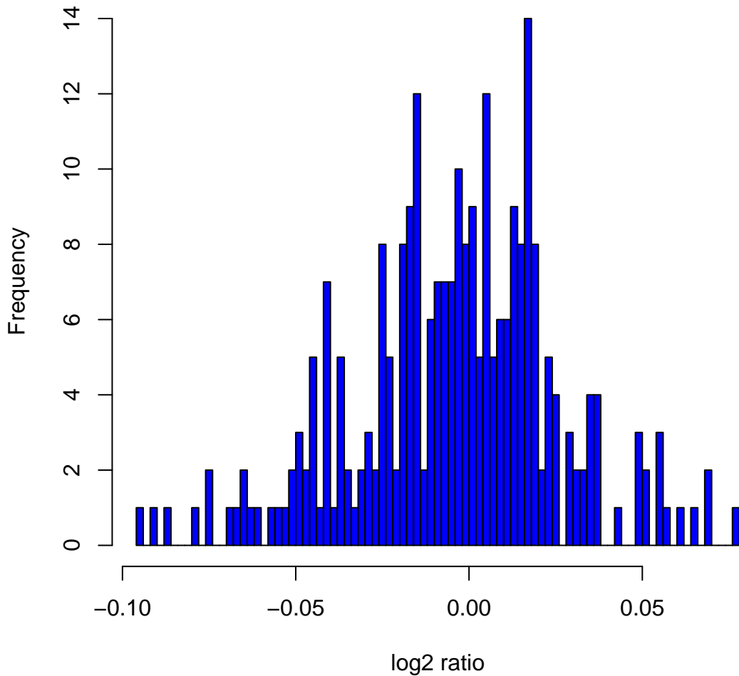
Histogram of \log_2 ratios in 270 HapMap samples at clone Chr9tp-1G3
