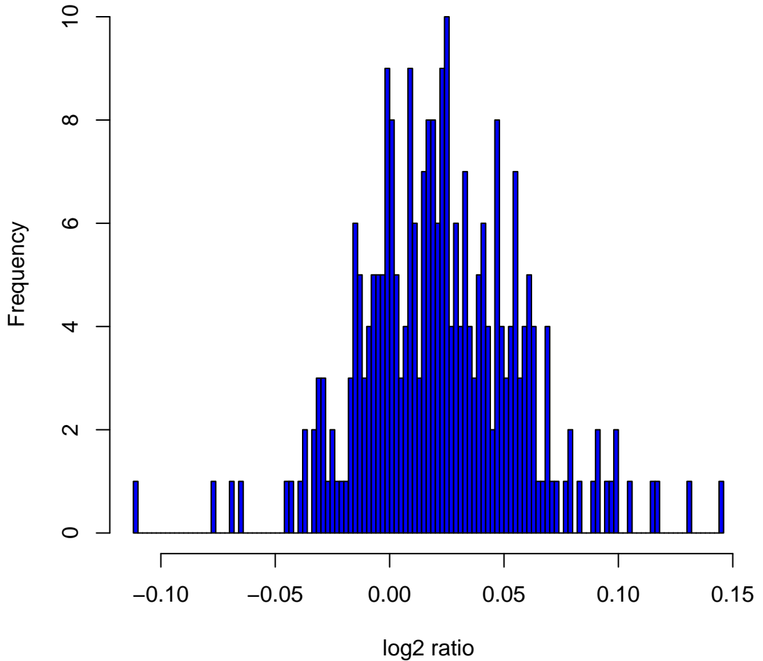
Histogram of log 2 ratios in 270 HapMap samples at clone Chr9tp-1H12
