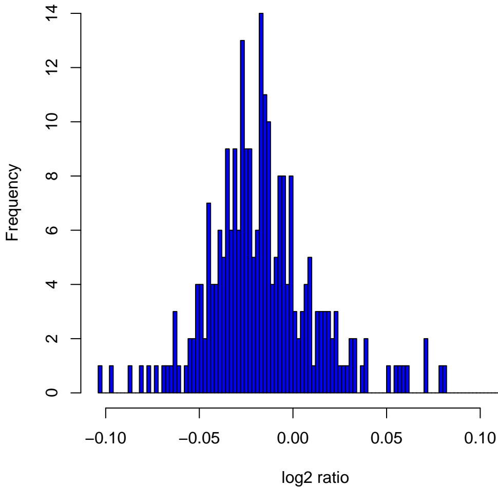
Histogram of log 2 ratios in 270 HapMap samples at clone Chr9tp-1H2
