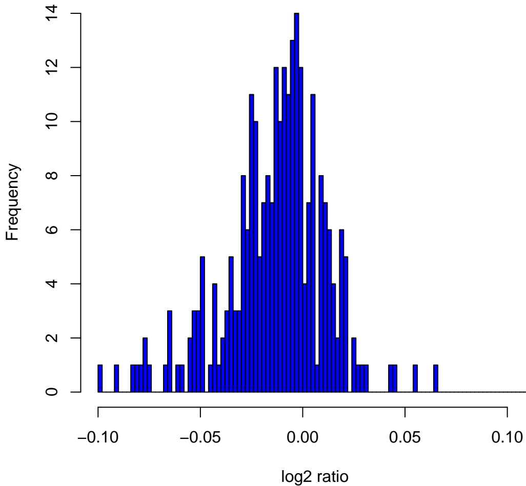
Histogram of \log_2 ratios in 270 HapMap samples at clone Chr9tp-1H3
