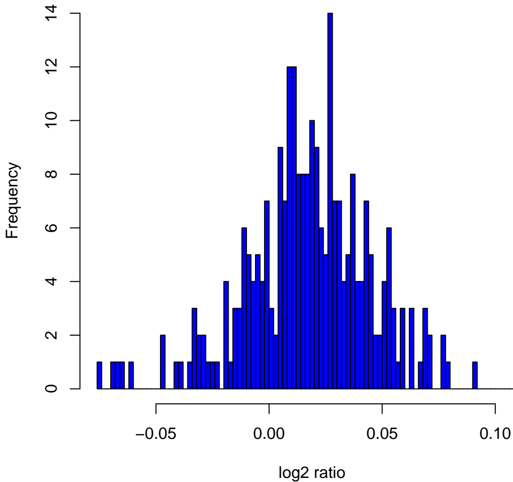
Histogram of log2ratios in 270 HapMap samples at clone Chr9tp-1H4
