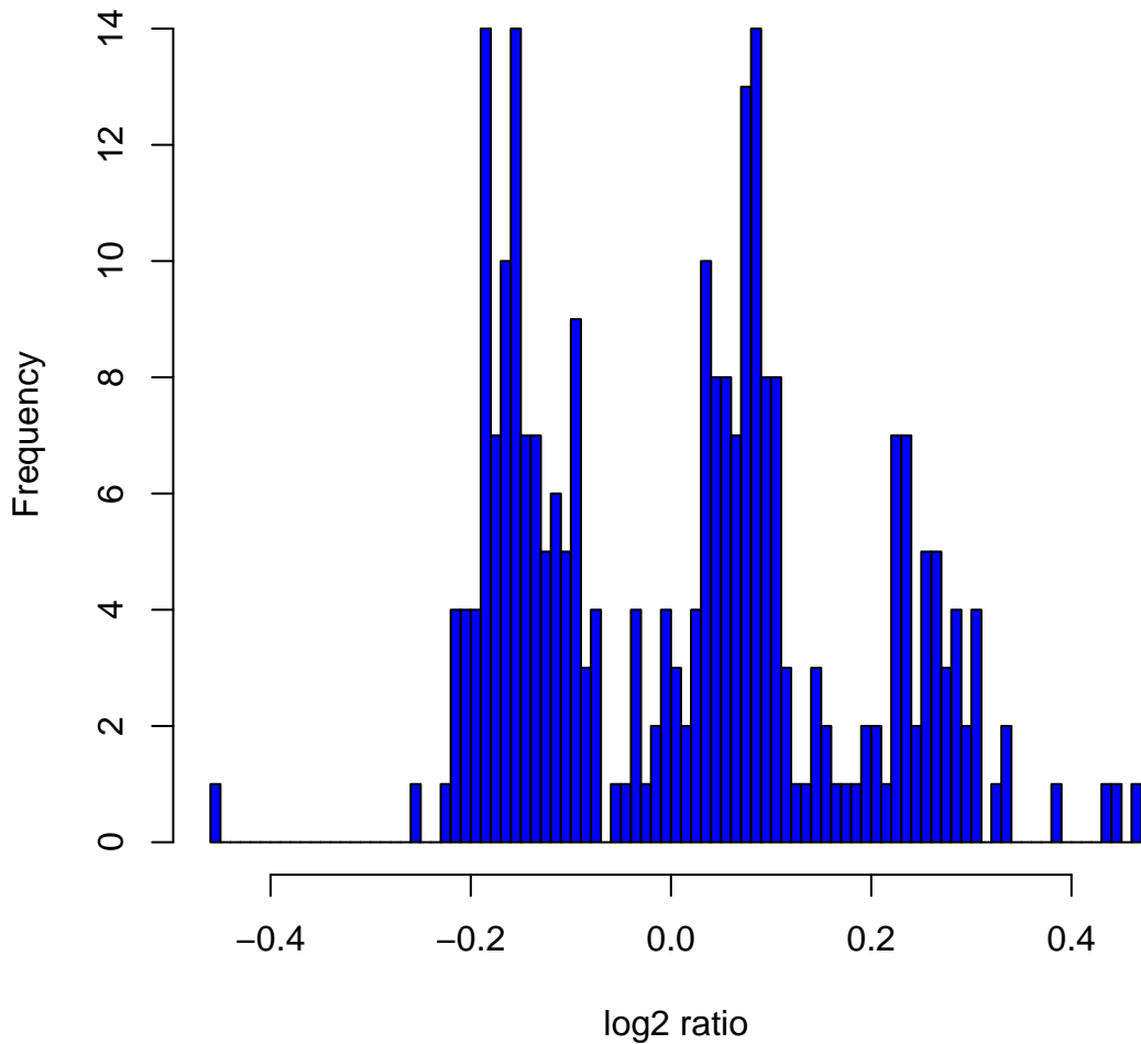
Histogram of log 2 ratios in 270 HapMap samples at clone Chr9tp-2A1
