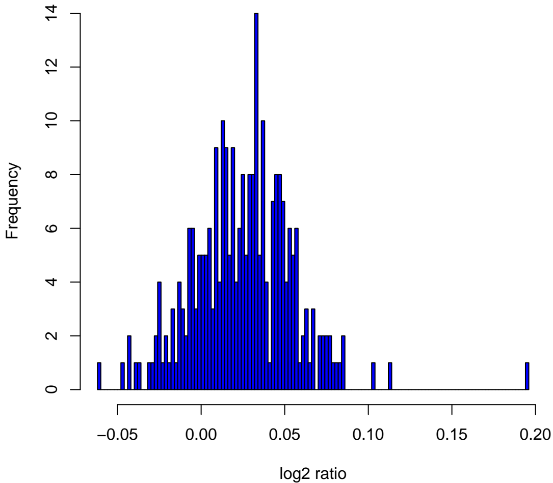
Histogram of log 2 ratios in 270 HapMap samples at clone Chr9tp-2B4
