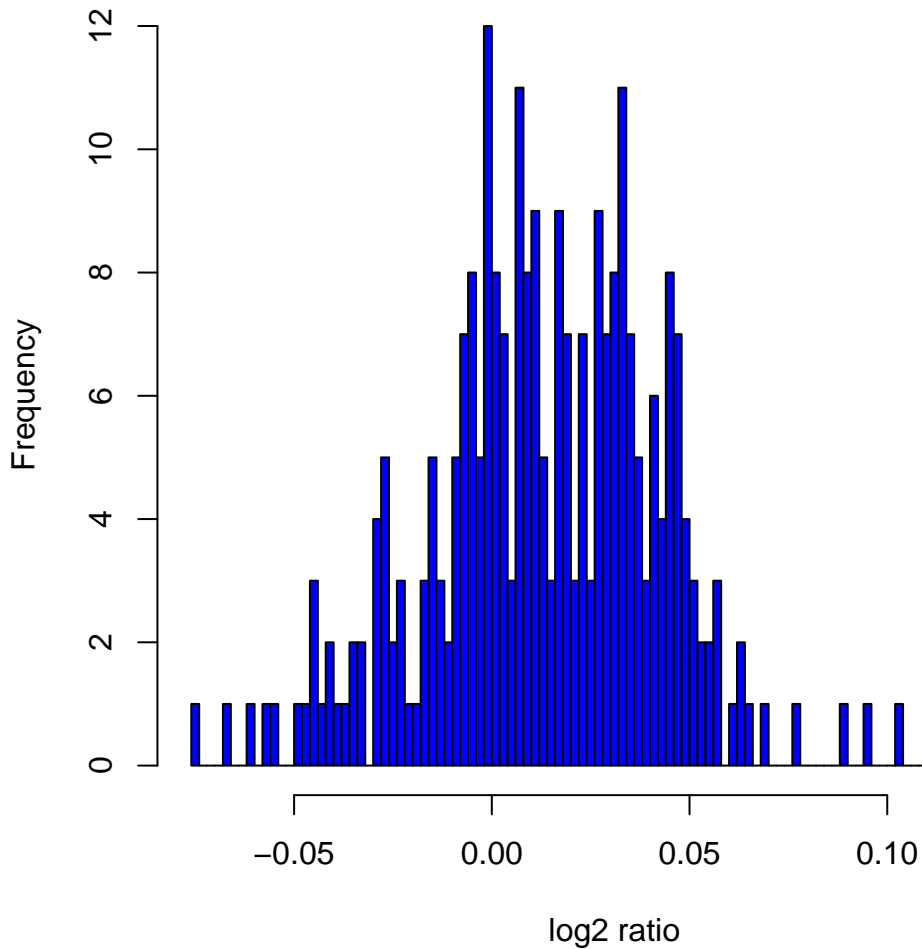
Histogram of \log_2 ratios in 270 HapMap samples at clone Chr9tp-2C10
