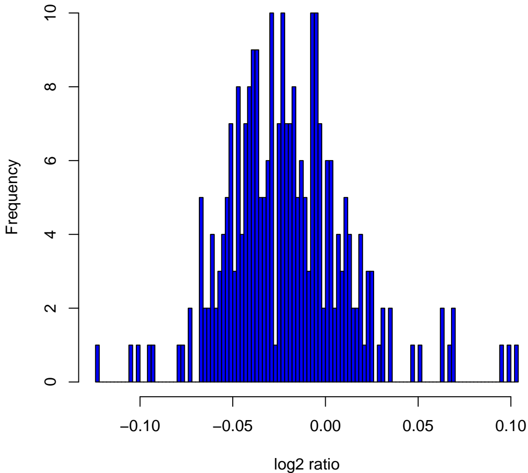
Histogram of log 2 ratios in 270 HapMap samples at clone Chr9tp-2C9
