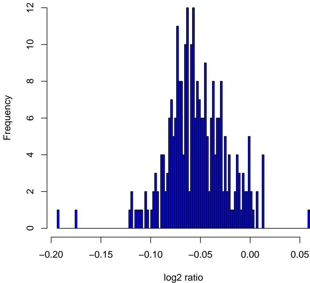
Histogram of log 2 ratios in 270 HapMap samples at clone Chr9tp-2E9
