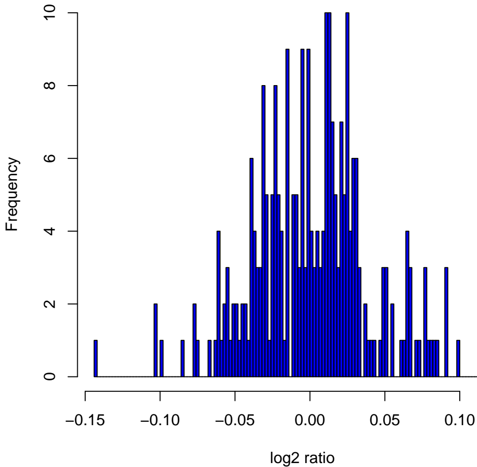
Histogram of log 2 ratios in 270 HapMap samples at clone Chr9tp-2F1
