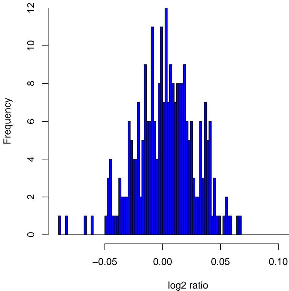
Histogram of log 2 ratios in 270 HapMap samples at clone Chr9tp-2F10
