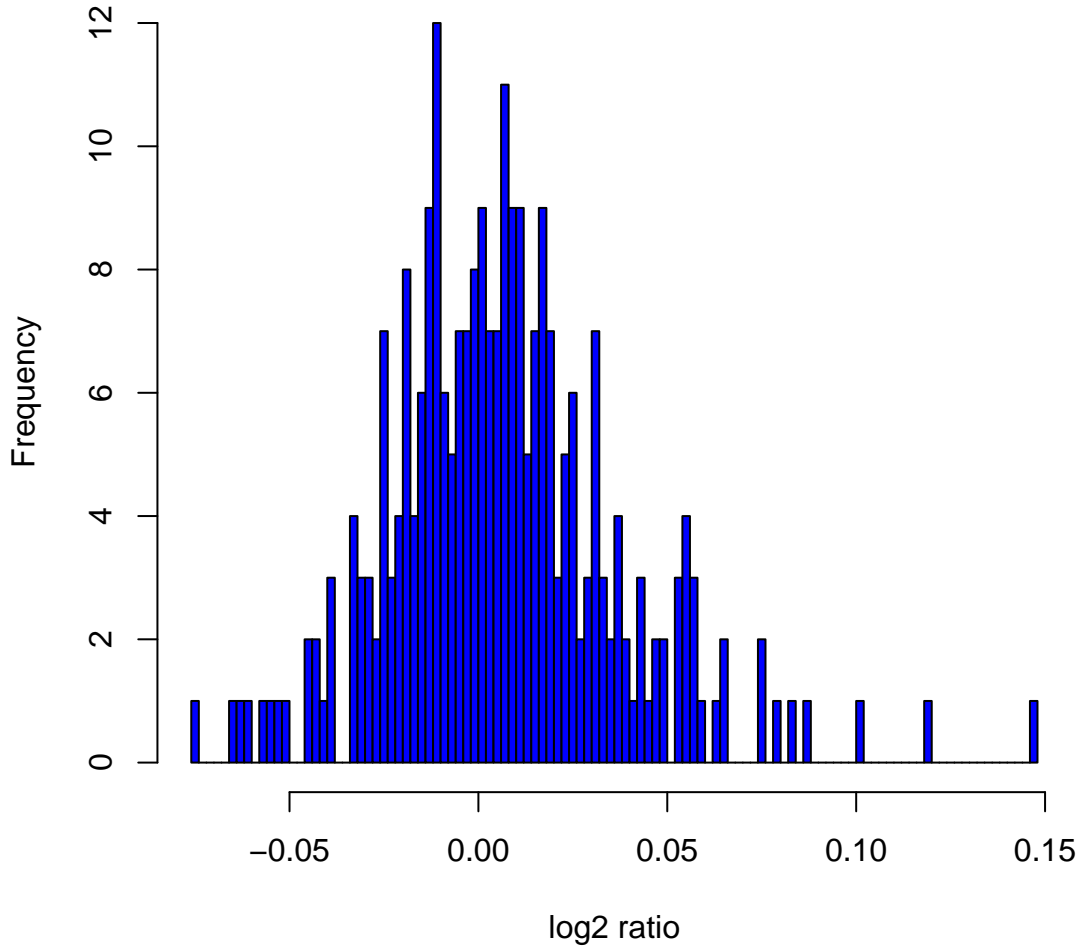
Histogram of log2ratios in 270 HapMap samples at clone Chr9tp-2F5
