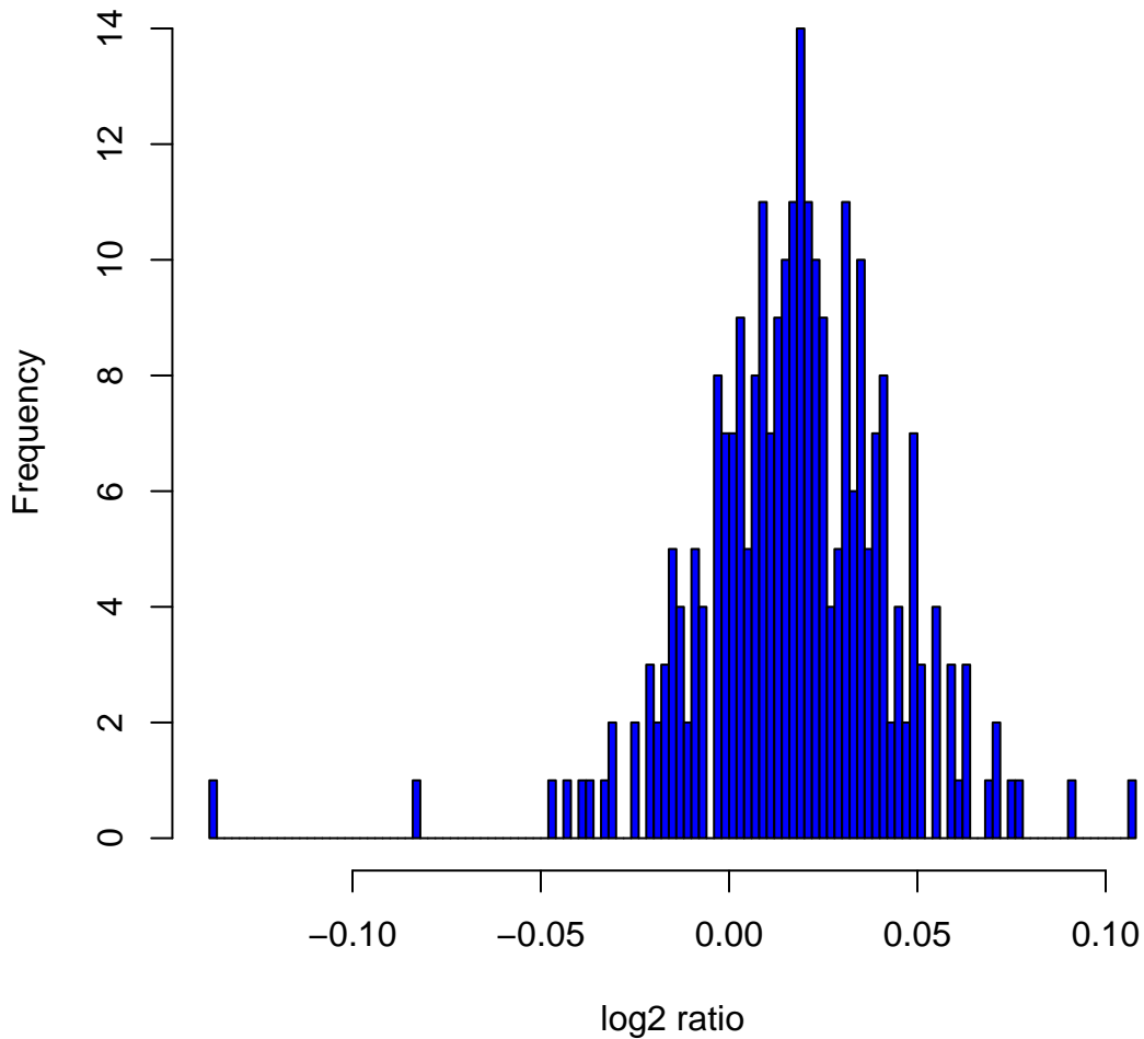
Histogram of log 2 ratios in 270 HapMap samples at clone Chr9tp-2G9
