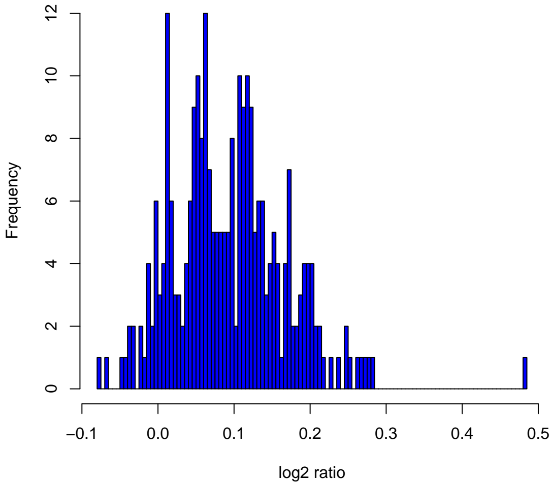
Histogram of log 2 ratios in 270 HapMap samples at clone Chr9tp-3A7
