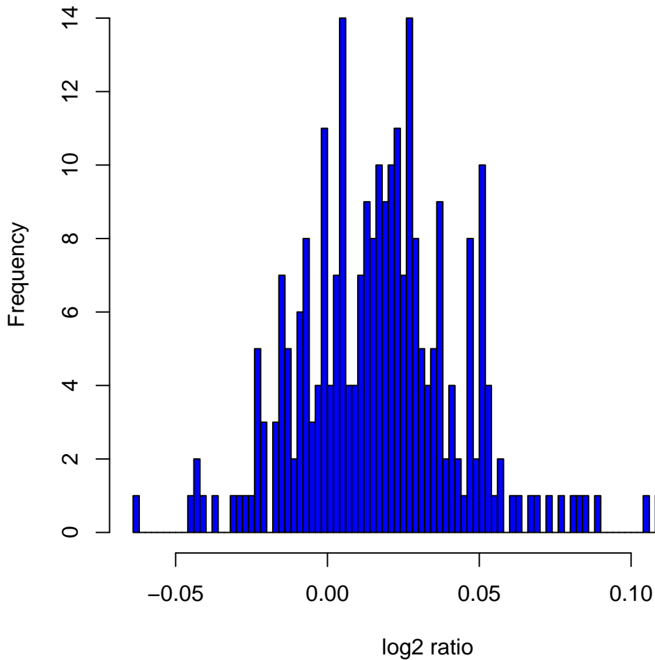
Histogram of \log_2 ratios in 270 HapMap samples at clone Chr9tp-3A8
