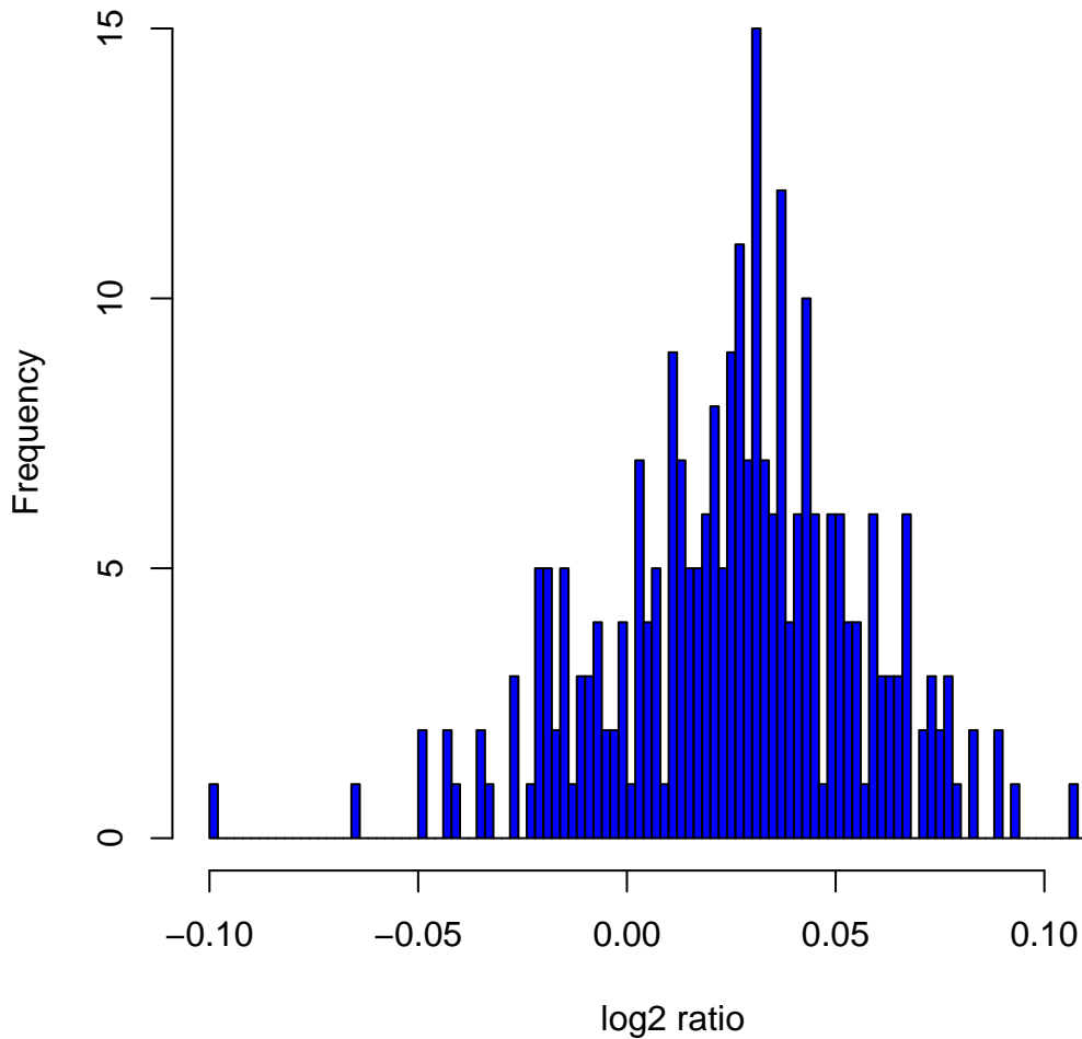
Histogram of log2ratios in 270 HapMap samples at clone Chr9tp-3E3
