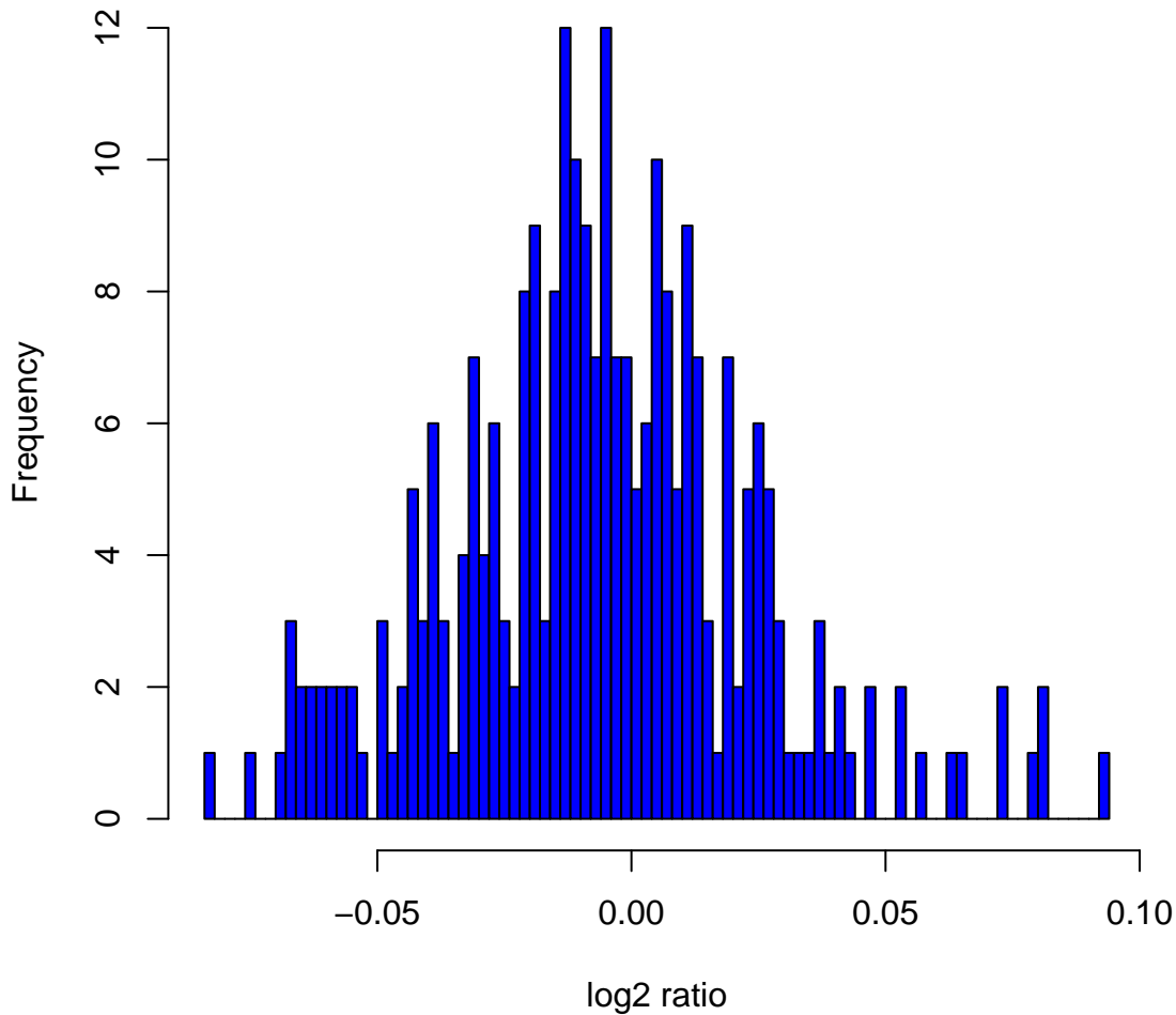
Histogram of log 2 ratios in 270 HapMap samples at clone Chr9tp-3E7
