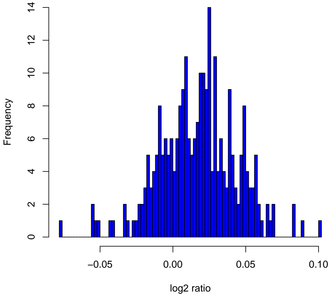
Histogram of log 2 ratios in 270 HapMap samples at clone Chr9tp-3F1
