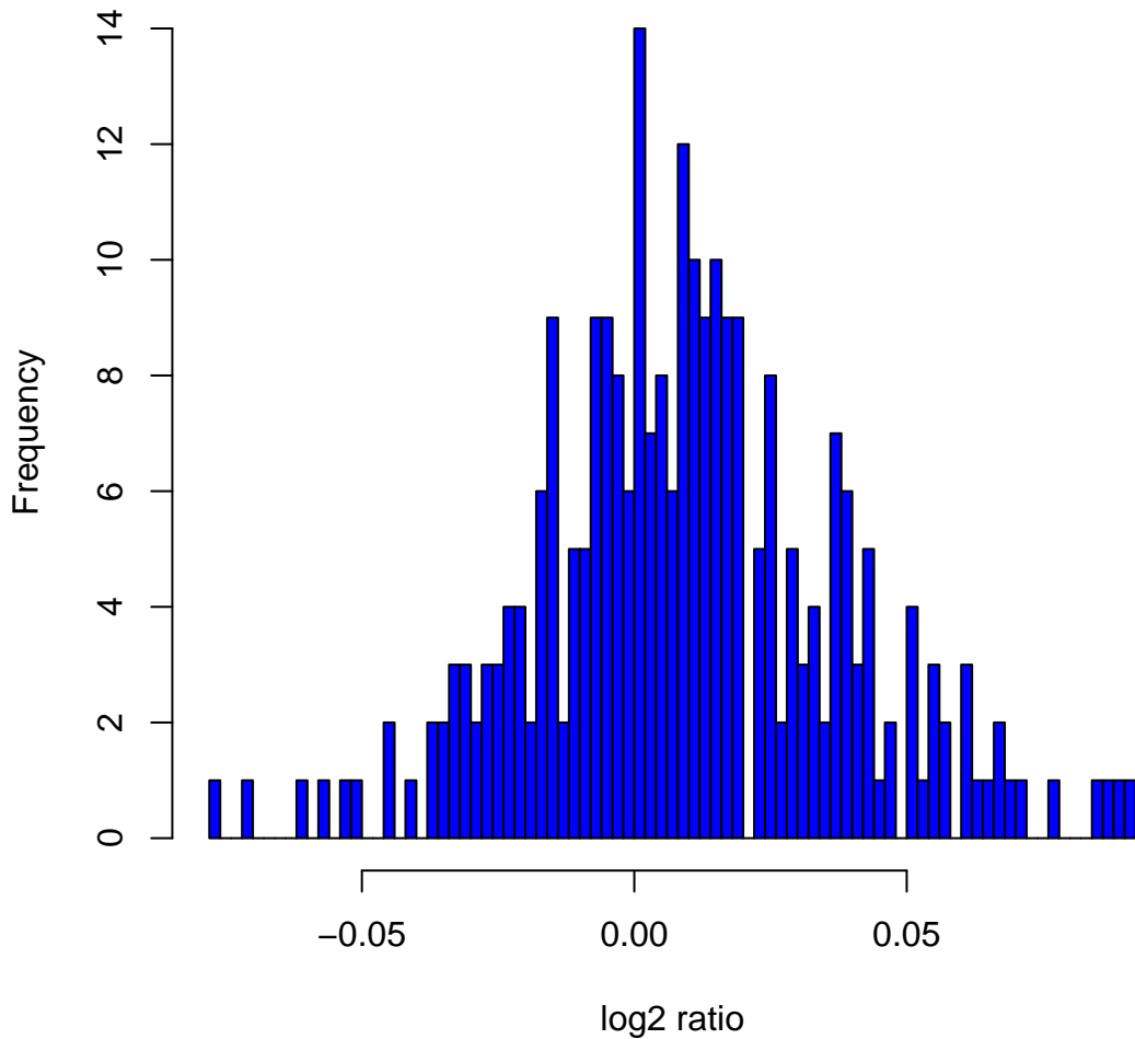
Histogram of log 2 ratios in 270 HapMap samples at clone Chr9tp-3F8
