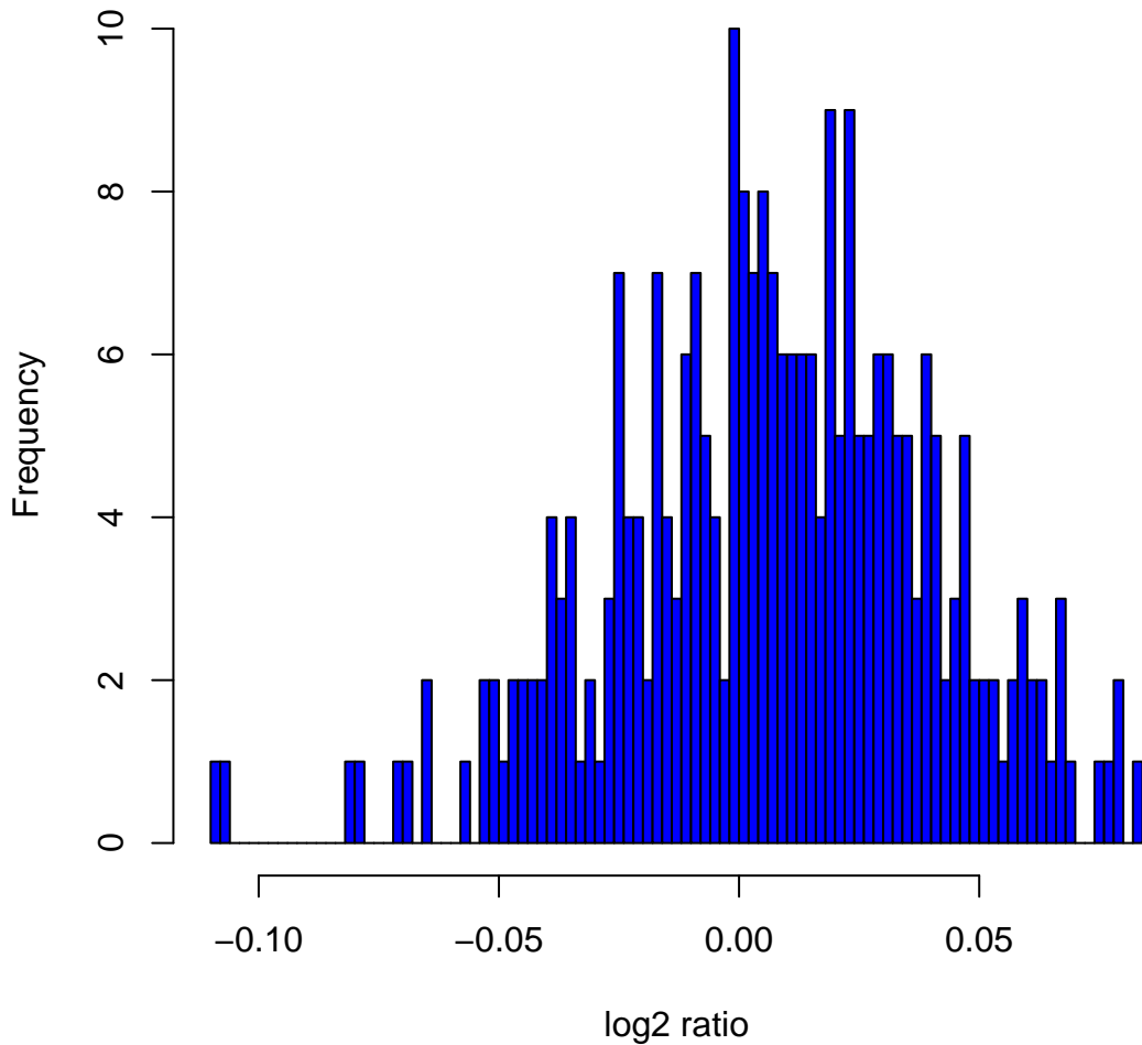
Histogram of log 2 ratios in 270 HapMap samples at clone Chr9tp-3H8
