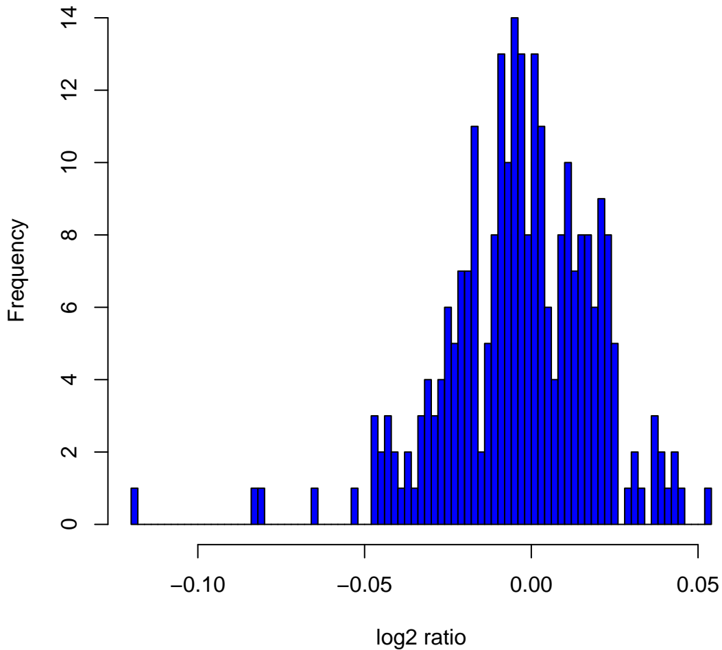
Histogram of log 2 ratios in 270 HapMap samples at clone Chr9tp-4A5
